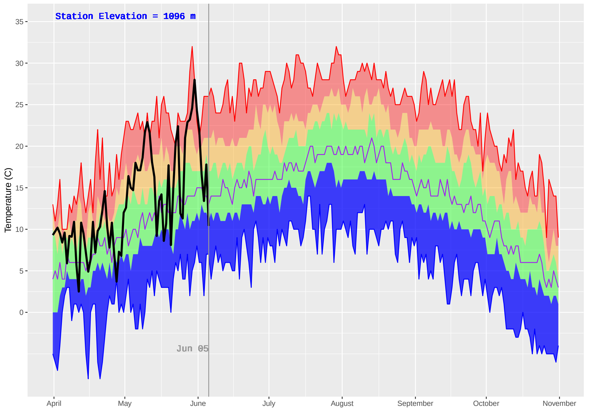
ANAHIM LAKE HUB (213) : Historical (1981–2018) and Current (2019) Daily Temperature
