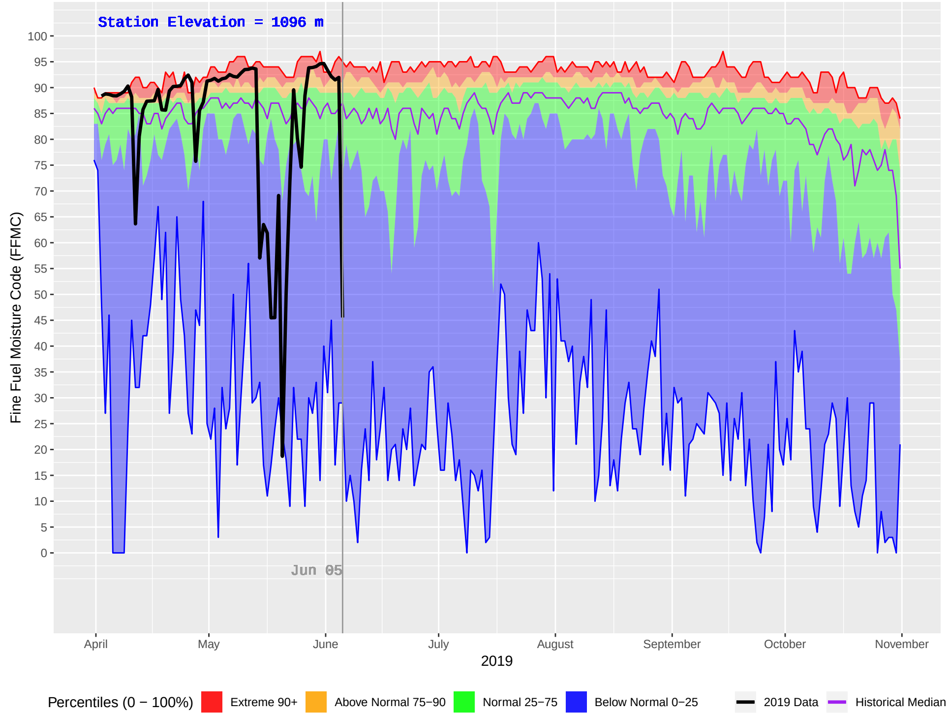
ANAHIM LAKE HUB (213) : Historical (1981–2018) and Current (2019) Daily Fine Fuel Moisture Code (FFMC)
