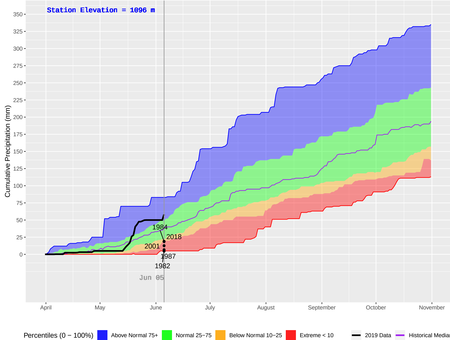
ANAHIM LAKE HUB (213) : Historical (1981–2018), Current (2019) Daily Cumulative Precipitation
