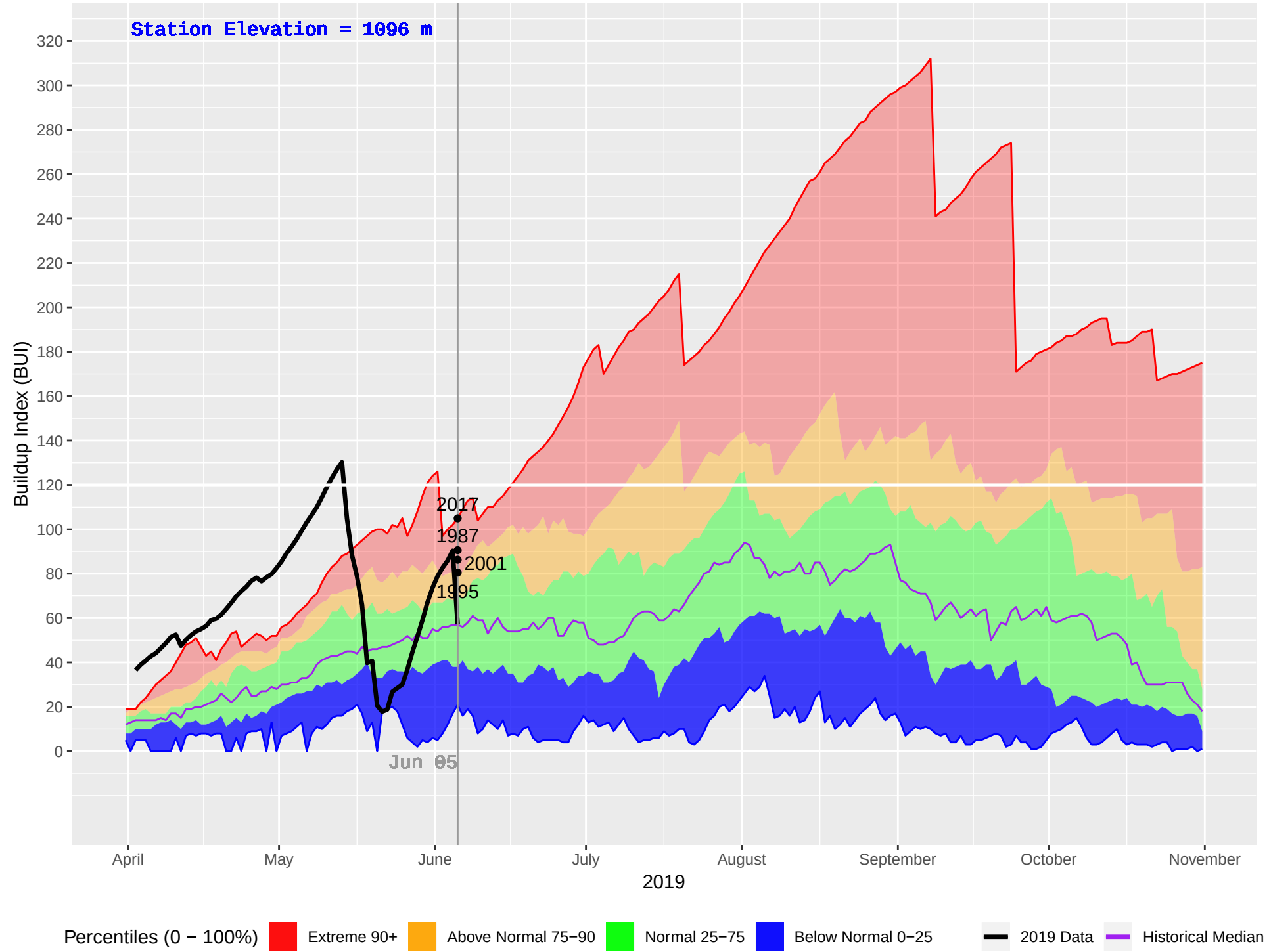
ANAHIM LAKE HUB (213) : Historical (1981–2018), Current (2019) Daily Buildup Index (BUI)
