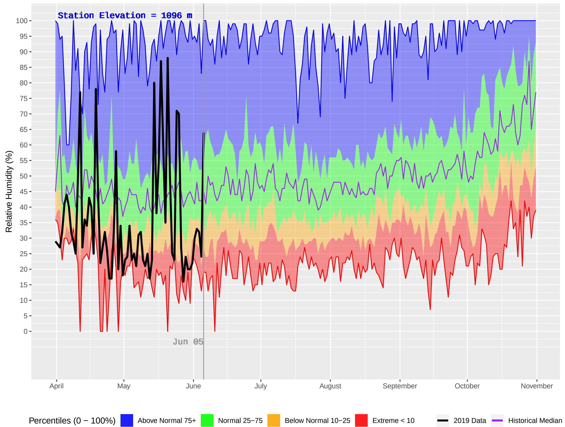
ANAHIM LAKE HUB (213) : Historical (1981–2018) and Current (2019) Daily Relative Humidity
