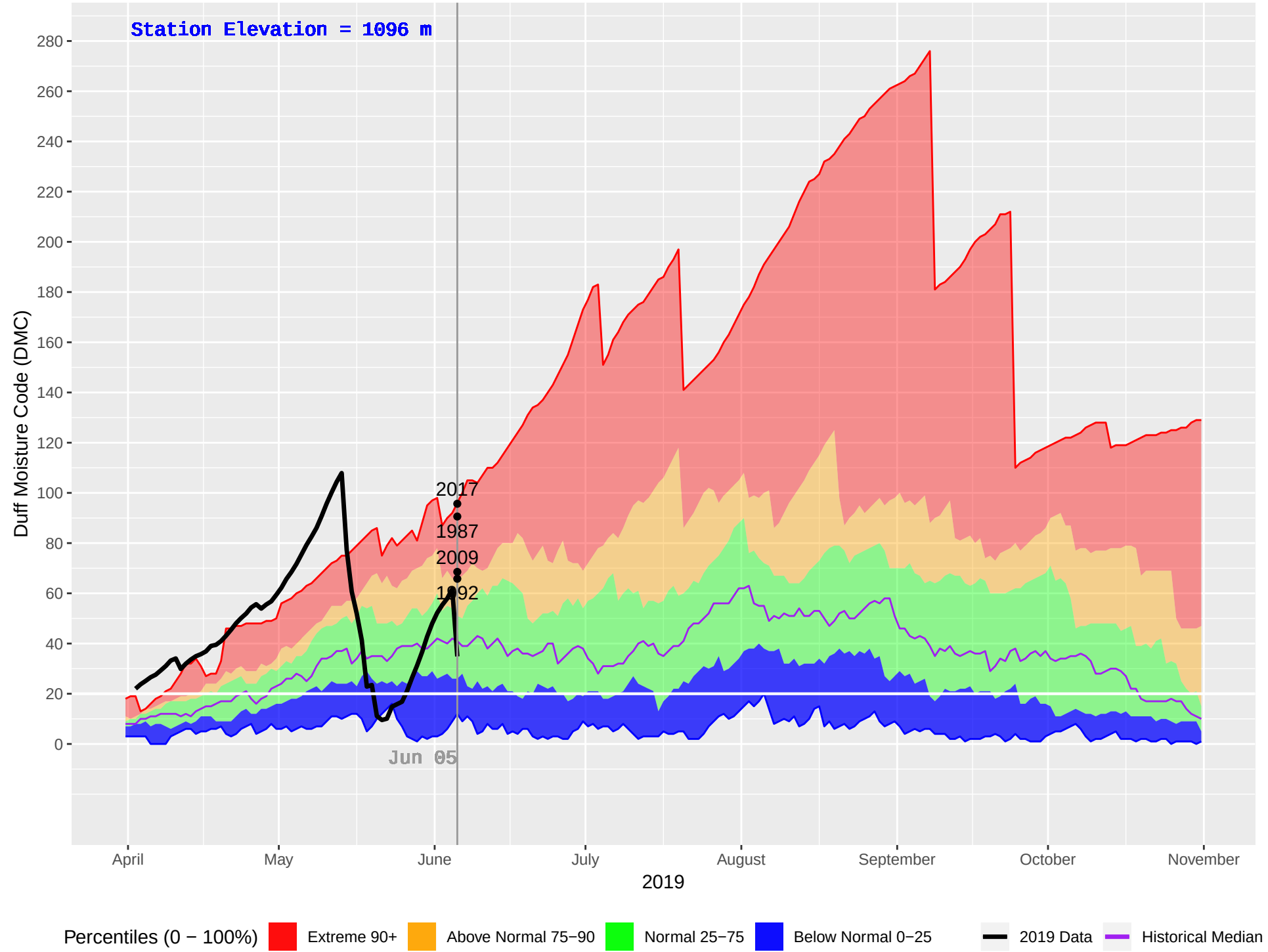
ANAHIM LAKE HUB (213) : Historical (1981–2018), Current (2019) Daily Duff Moisture Code (DMC)
